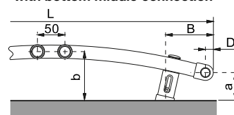
KRM, KRC, KRT without bottom middle connection
