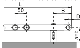
KLM, KLC, KLT without bottom middle connection
