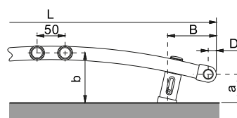
KRM, KRC, KRT sans raccordement central
