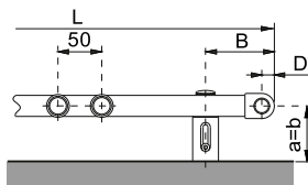
KLM, KLC, KLT sans raccordement central
